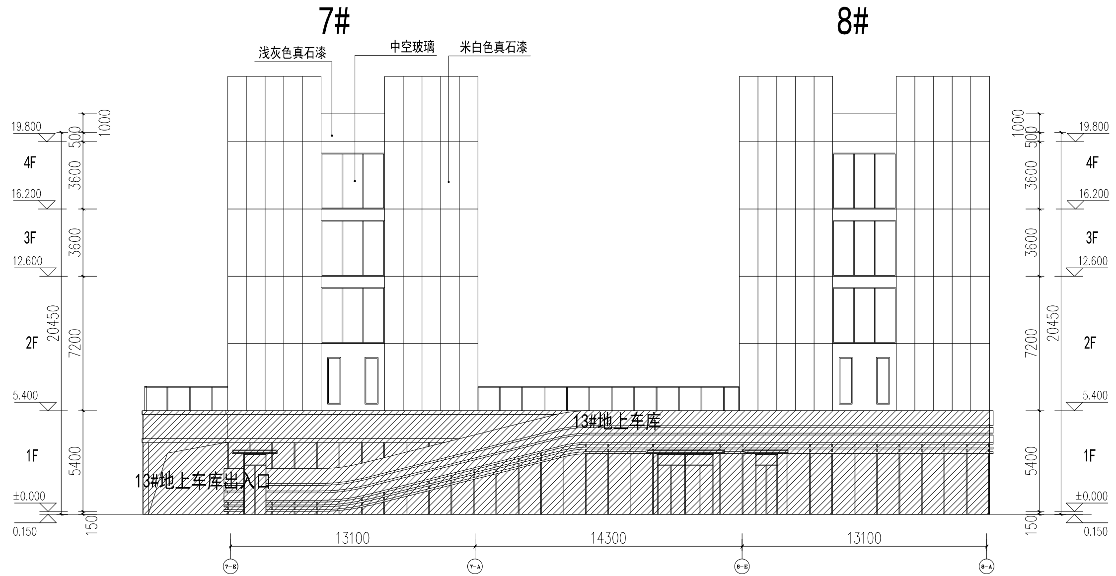
7#8#西立面图
